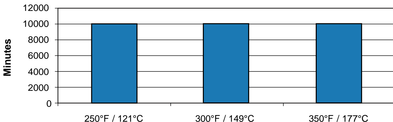
Chart #2 Static Shear of 3M™ Extreme Sealing Tape 4412N at Elevated Temperatures ASTM D-3654 (1" x 1", 100 grams, stainless steel) Panel Prep: 1 wipe 50/50 IPA/water; Prime with 3M™ Adhesion Promoter 111
